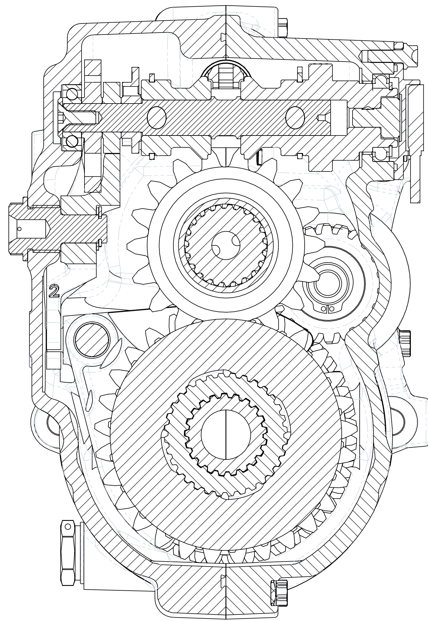
SECTION C-C
